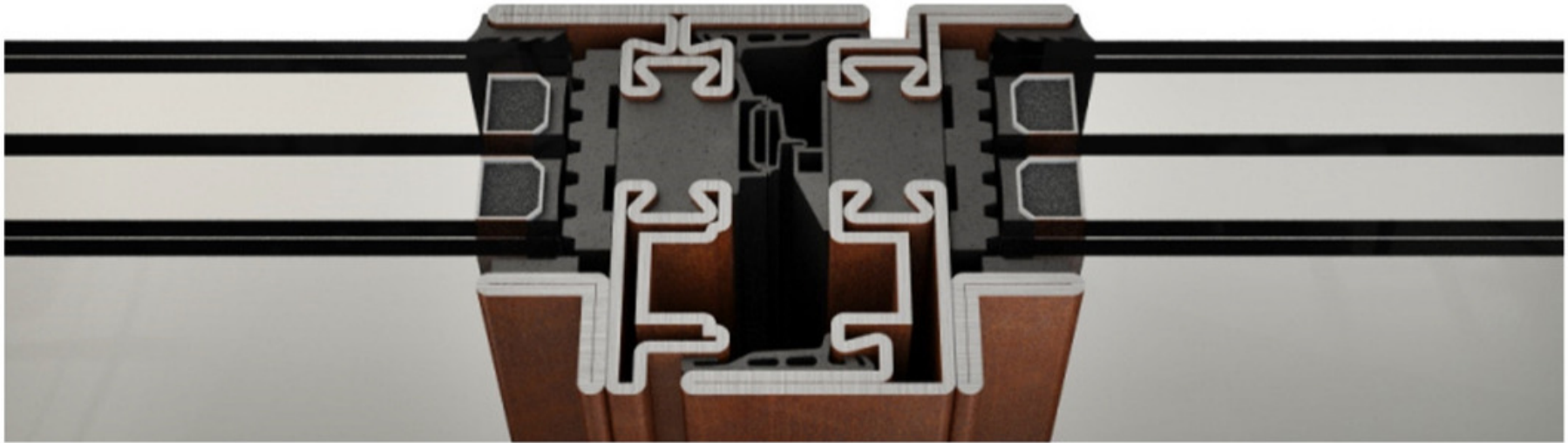
Middle frame
